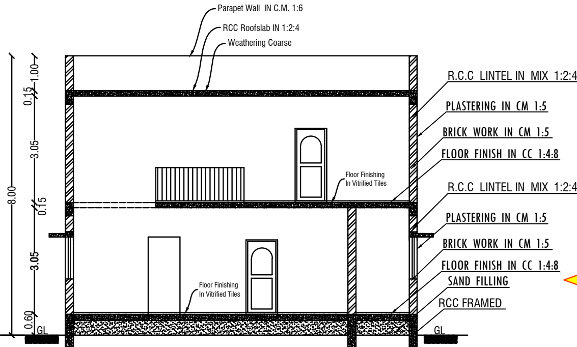
SECTION -AA
