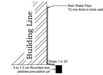
RAINWATER HARVESTING
