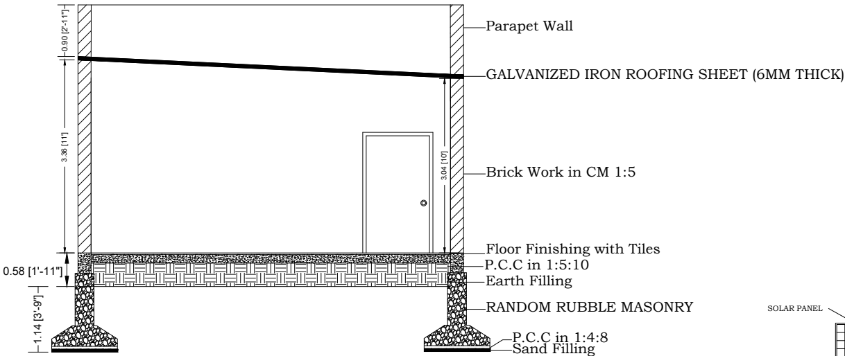
SECTION X-X
