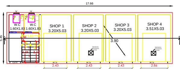
PROPOSED GROUND FLOOR PLAN
