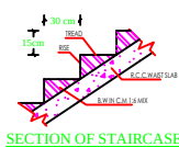
SECTION OF STAIRCASE
