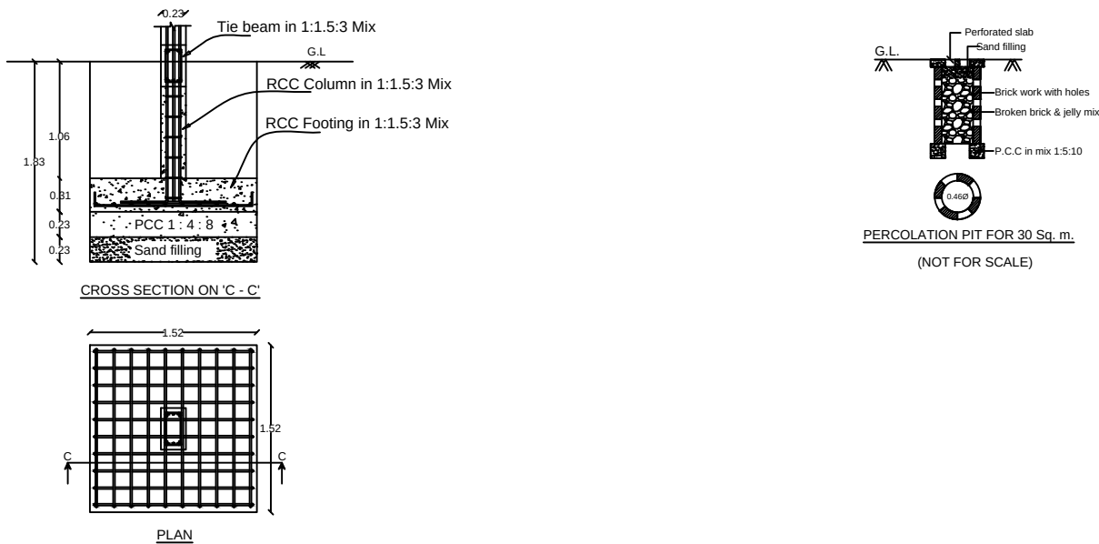
COLOUMN FOUNDATION DETAILS
