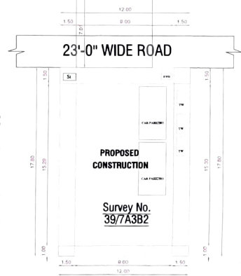
Sundaram's Land SITE PLAN (SCALE 1:100)
