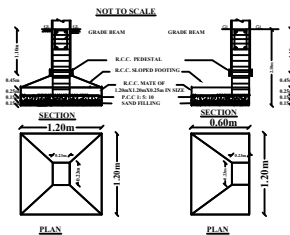
COLUMN FOOTING DETAILS
