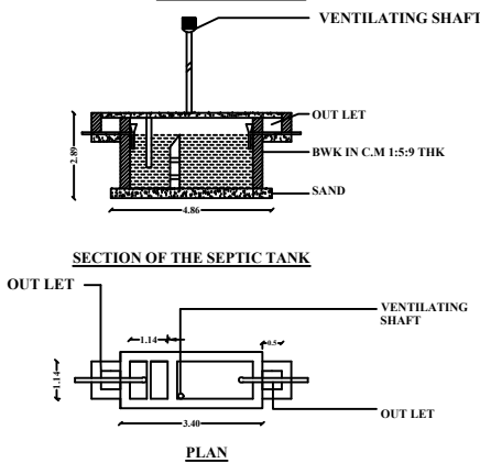
SEPTIC TANK
