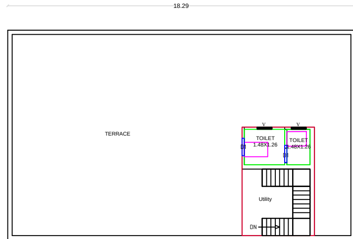
PROPOSED SECOND FLOOR PLAN
