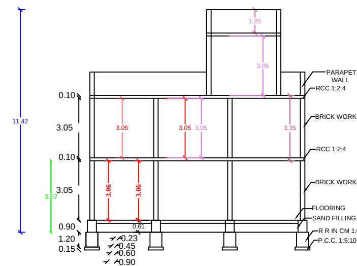
SECTION AB
