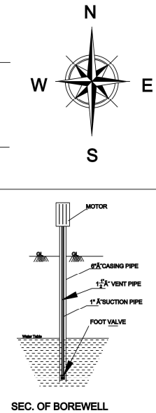
SEC. OF BOREWELL
