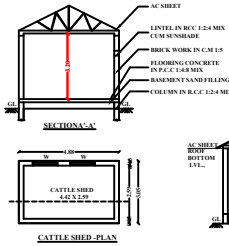
CATTLE SHED PLAN
