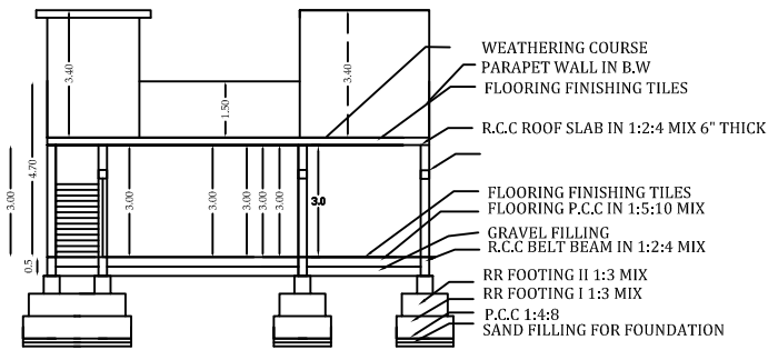
SECTION A TO B
