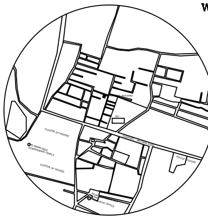
TOPO PLAN:- (SCALE 1:1000)
