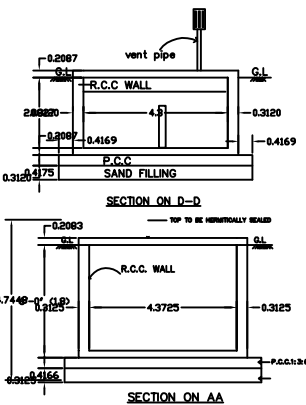
SECTION ON D-D
