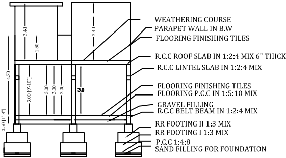
SECTION A TO B
