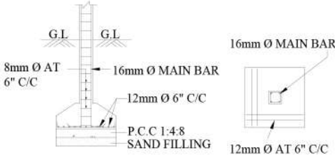
Column Footing Details: Column size - 9" x 12"
