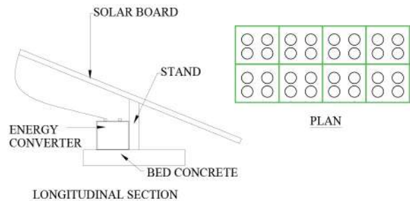
SOLAR SYSTEM
