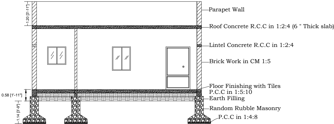
SECTION X-X
