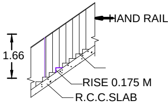
STAIRCASE
