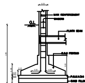
TYPICAL SECTION OF R.C.C COLUMN FOUNDATION
