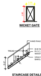
STAIRCASE DETAILS
