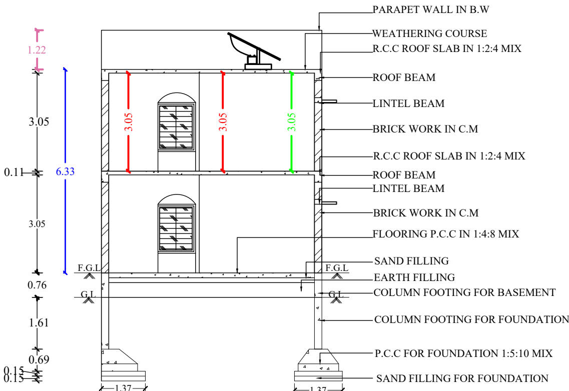
SECTION ON-AA
