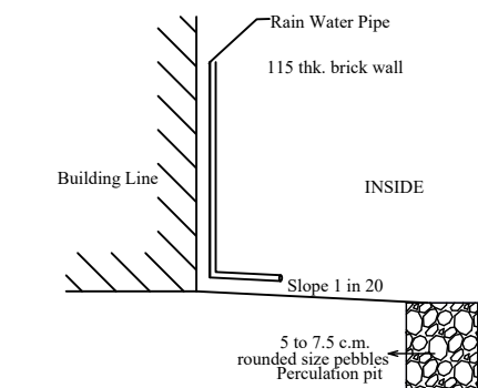
PERCOLATION PIT :
