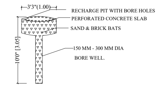
RAINWATER HARVESTING:-
