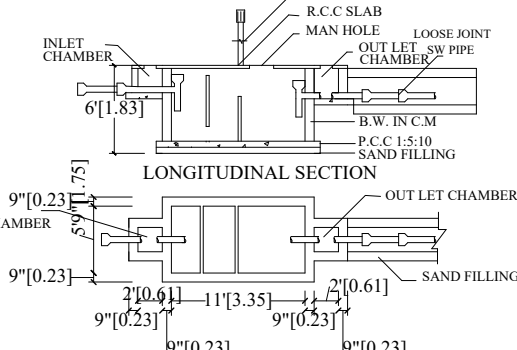
SEPTIC TANK:-
