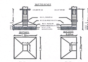
COLUMN FOOTING DETAILS
