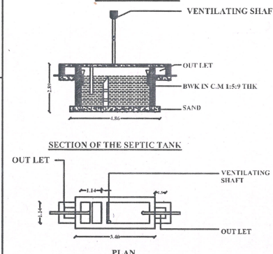
SEPTIC TANK
