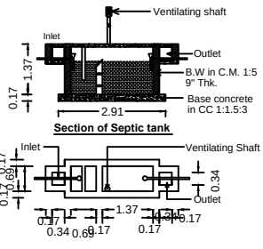
SEPTIC TANK DETAIL
