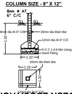
COLUMN FOOTING DETAILS
