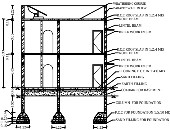
SECTION ON-AA
