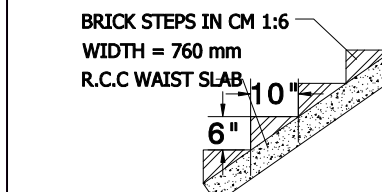
STAIRCASE DETAILS (NOT TO SCALE)
