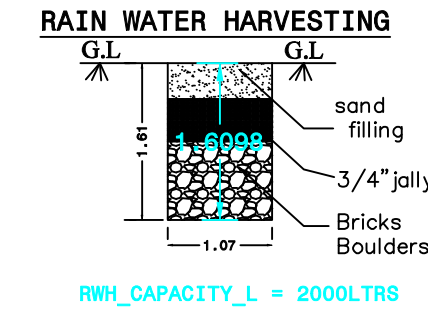
RWH_CAPACITY_L = 2000LTRS
