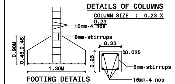
FOOTING DETAILS
