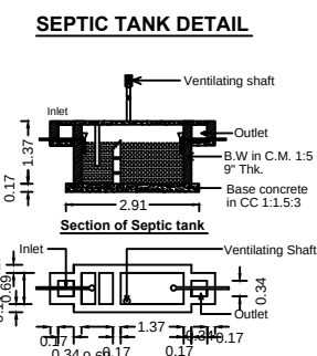
SEPTIC TANK DETAIL
