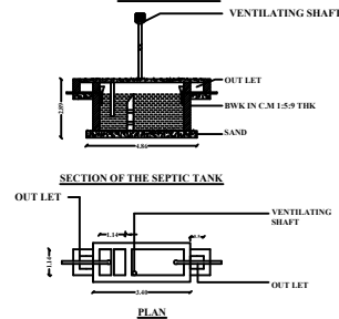
SEPTIC TANK
