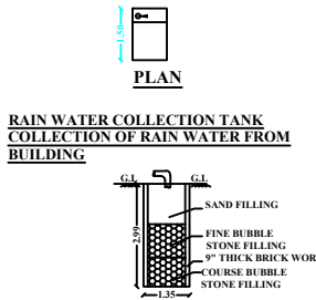
SECTION ON RAIN WATER COLLECTION TANK
