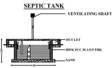
SECTION OF THE SEPTIC TANK
