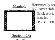
Section On [XZ, XZ]
