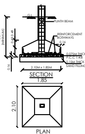
FOUNDATION DETAILS
