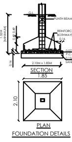
FOUNDATION DETAILS
