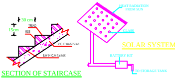
SECTION OF STAIRCASE
