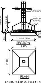
FOUNDATION DETAILS
