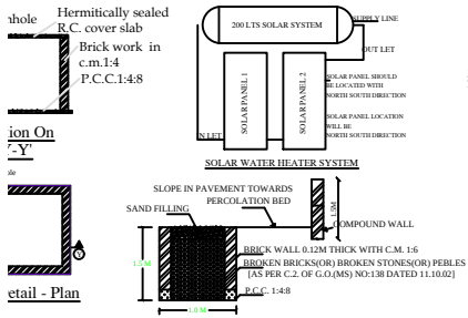
SECTION OF RAIN WATER PERCOLATION BED
