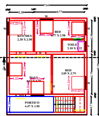
FIRST FLOOR
