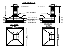
COLUMN FOOTING DETAILS
