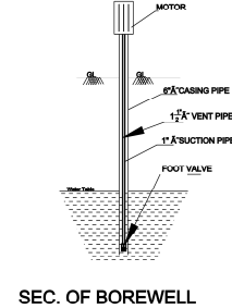
SEC. OF BOREWELL
