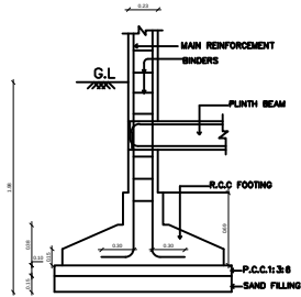
TYPICAL SECTION OF R.C.C COLUMN FOUNDATION
