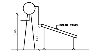
SIDE ELEVATION (NOT TO SCALE)
