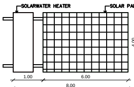
PLAN OF SOLAR PANEL & SOLAR WATER HEATER (NOT TO SCALE)
