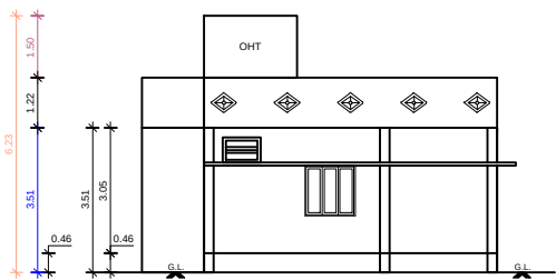
SOUTH ELEVATION
