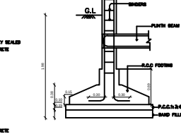
TYPICAL SECTION OF R.C.C COLUMN FOUNDATION
