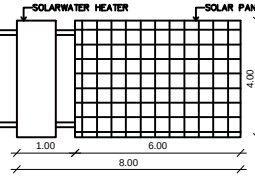
PLAN OF SOLAR PANEL & SOLAR WATER HEATER (NOT TO SCALE)
