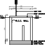
SECTION ON CC
