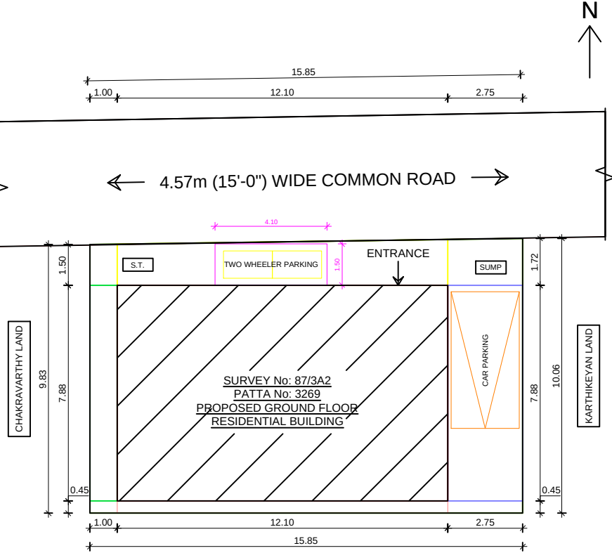
SITE PLAN
