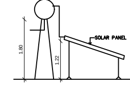
SIDE ELEVATION (NOT TO SCALE)
