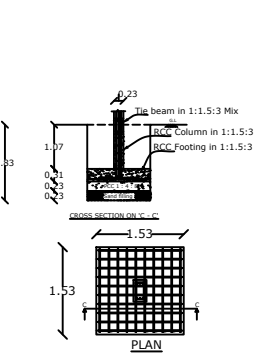
COLUMN FOUNDATION DETAILS:-
