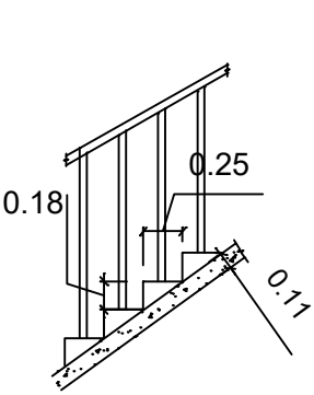
STAIRCASE DETAILS:-
