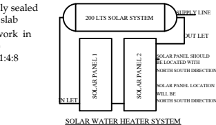
SOLAR WATER HEATER SYSTEM
