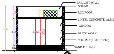
SECTION ON A-B
