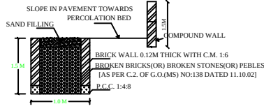
SECTION OF RAIN WATER PERCOLATION BED
