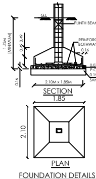
FOUNDATION DETAILS
