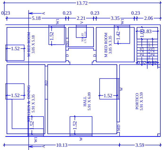
PLAN FOR GROUND FLOOR
