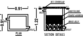
RAINWATER HARVESTING SYSTEM
