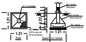
FOOTING DETAILS
