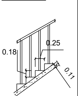
STAIRCASE DETAILS:-
