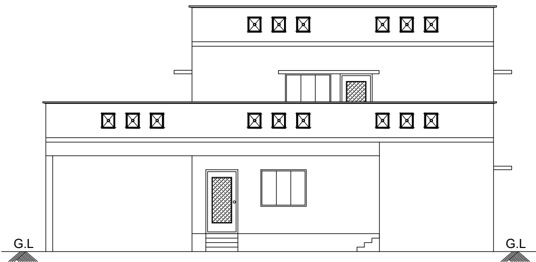
FRONT ELEVATION
