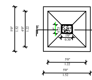
Footing & Column
