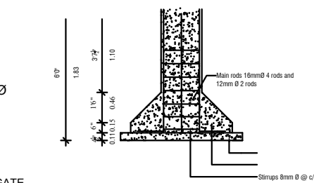
SECTION ON - " FF "
