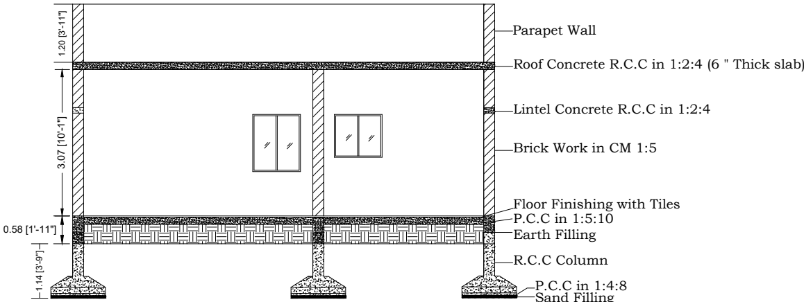
SECTION X-X
