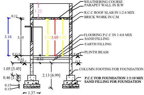
SECTION ON-AA
