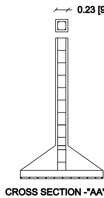
COLUMN DETAILS :-
