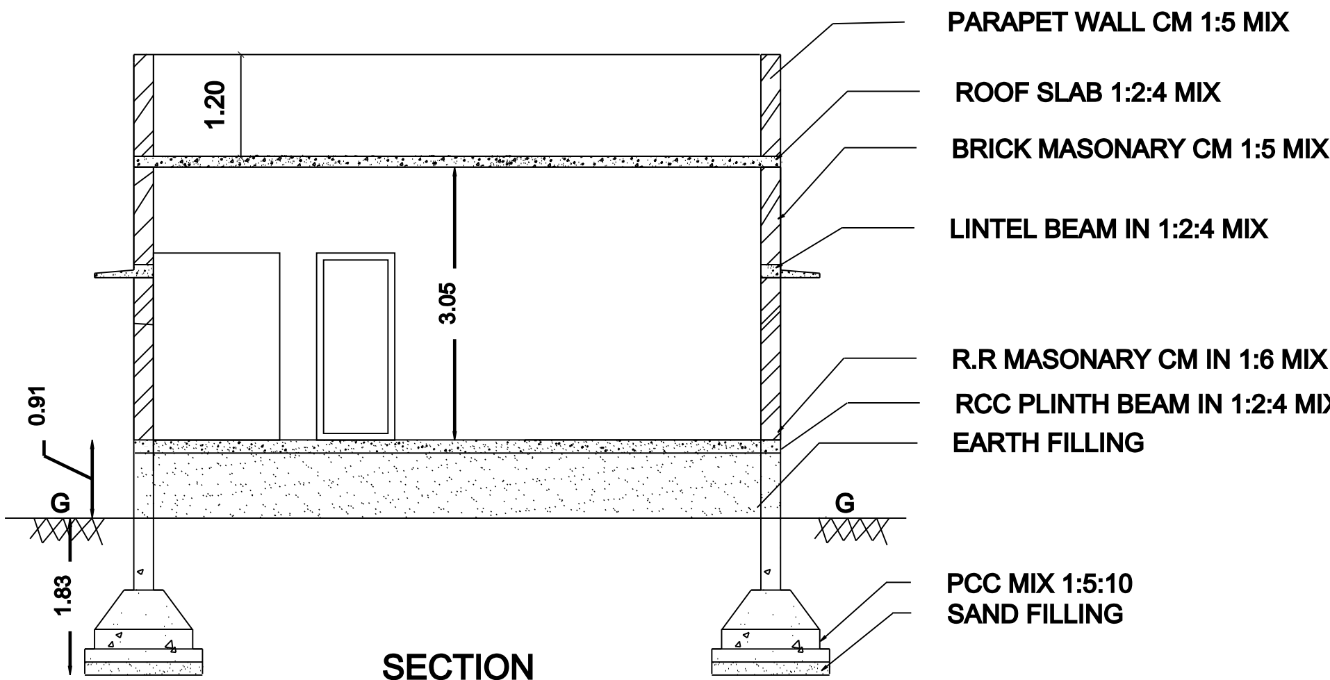
SECTION
