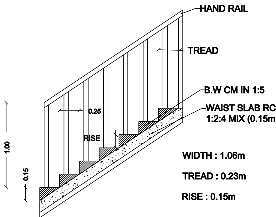
STAIRCASE DETAILS :-
