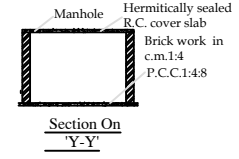
SECTION OF RAIN WATER PERCOLATION BED
