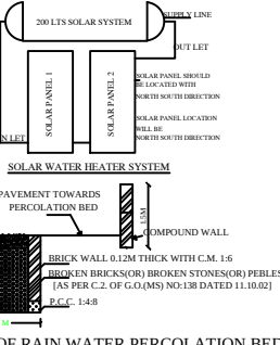
SECTION OF RAIN WATER PERCOLATION BED
