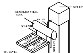
SOLAR HEATING WATER SYSTEM
