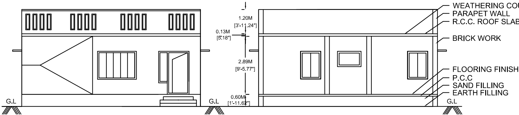
FRONT ELEVATION
