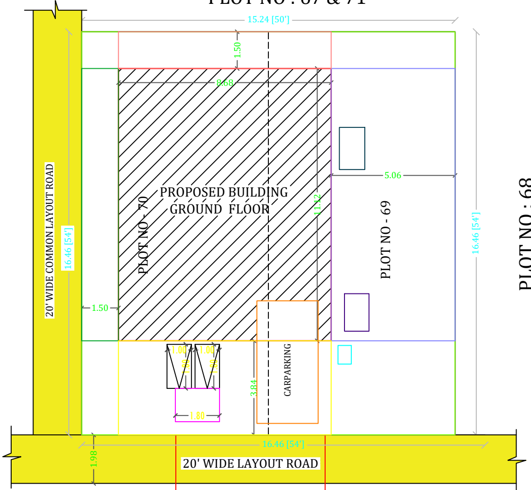
SITE PLAN
