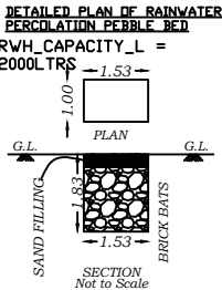
DETAILED PLAN OF RAINWATER PERCOLATION PEBBLE BED
