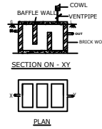
SEPTICTANK DETAILS NOT TO SCALE
